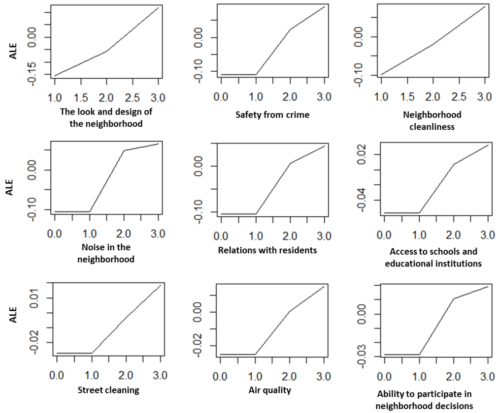
Figure S1 Accumulative Local Effects (ALE) Plots of Influential Contributors to Neighborhood Satisfaction
