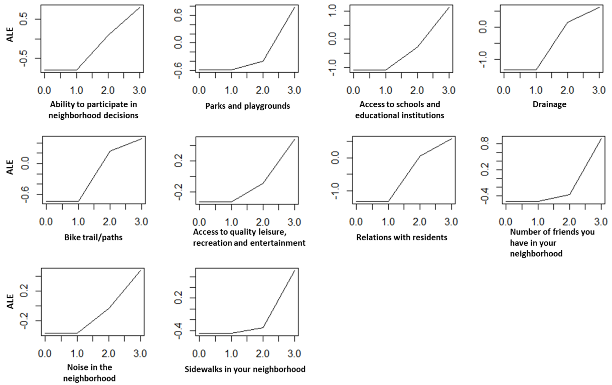
Figure S2 Accumulative Local Effects (ALE) Plots of Influential Contributors to Life Satisfaction
