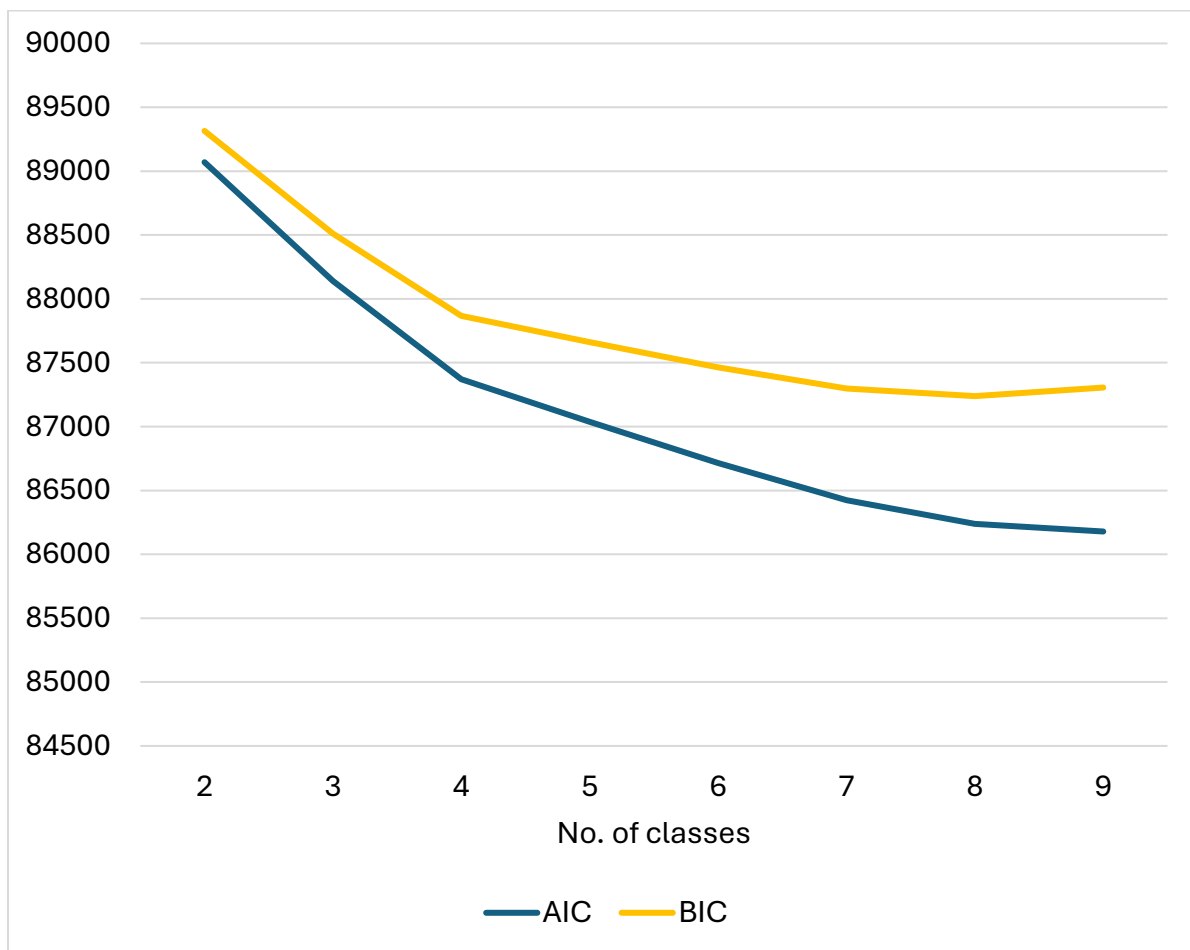
Figure 1. Model diagnostics
