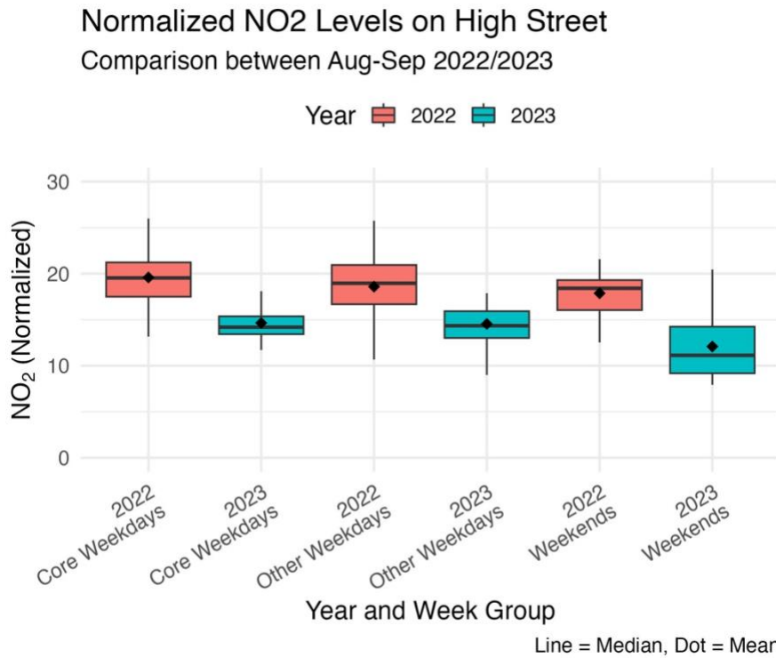
Figure 3 Normalized NO 2 levels on High Street during pre-LEZ (2022) and post-LEZ (2023) across the days of the week
