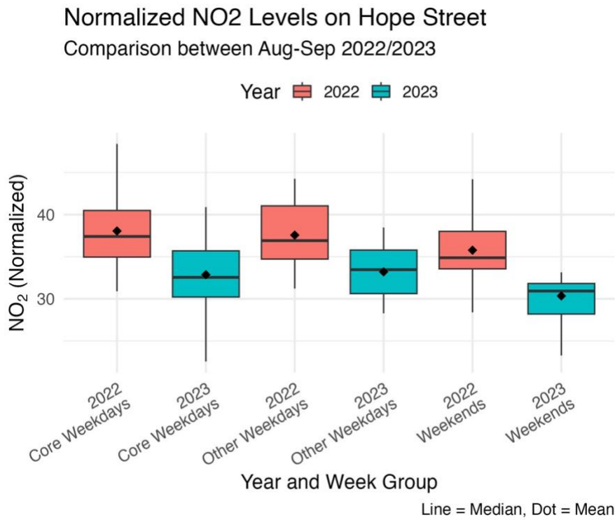
Figure 4 Normalized NO 2 levels on Hope Street during pre-LEZ (2022) and post-LEZ (2023) across the days of the week
