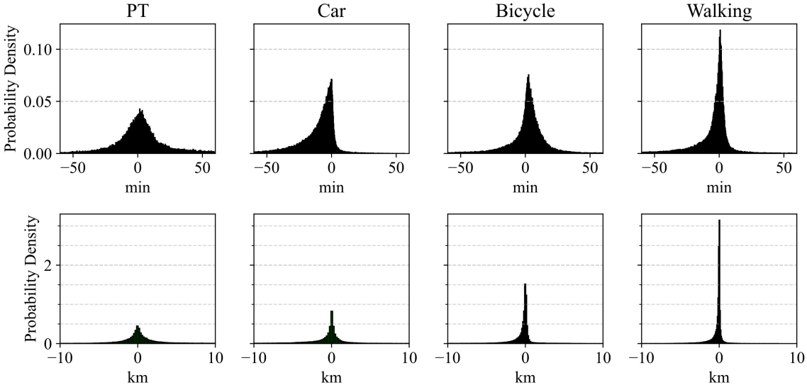
Fig. 1. Analysis of deviations of distance and duration between recorded trips and routed trips for different modes.
